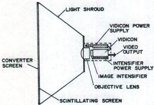
Fig. 59. Schematic of radiographic imaging unit.
